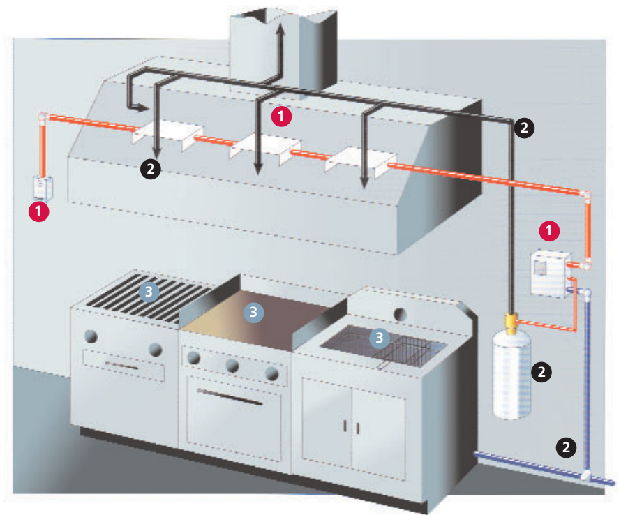
How the Kidde Fire Protection Wet Chemical system works:
